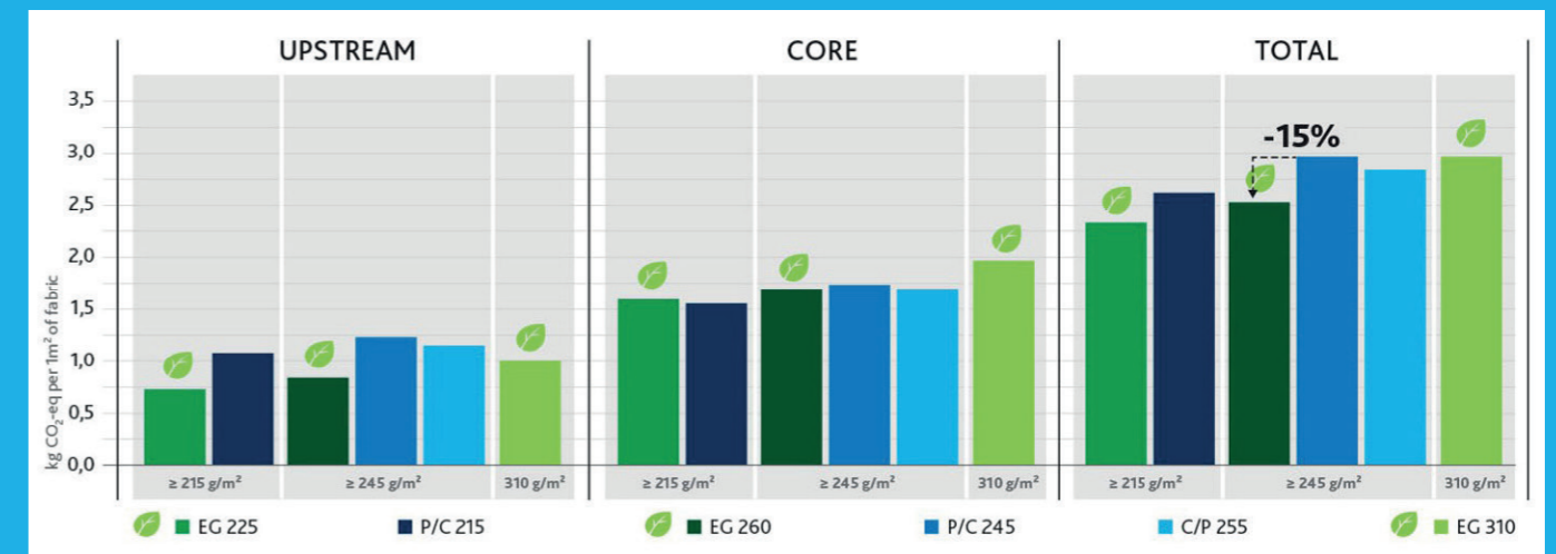
Figure 4. The Global Warming Potential of Tecawork™ Ecogreen fabrics EG 225, EG 260, EG 310 compared to poly-cotton fabrics P/C 215, P/C 245 and C/P 255. Figures for one square meter fabric.
