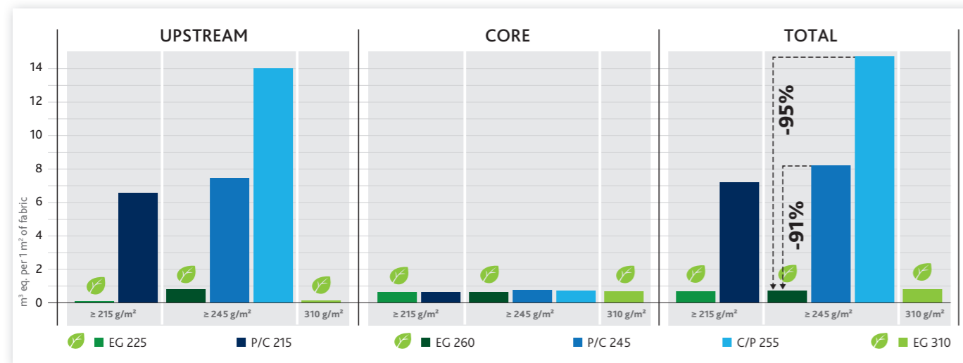
Figure 2. The Water Scarcity Footprint of Tecawork™ Ecogreen fabrics EG 225, EG 260, EG 310 compared to poly-cotton fabrics P/C 215, P/C 245 and C/P 255. Figures for one square meter fabric.
