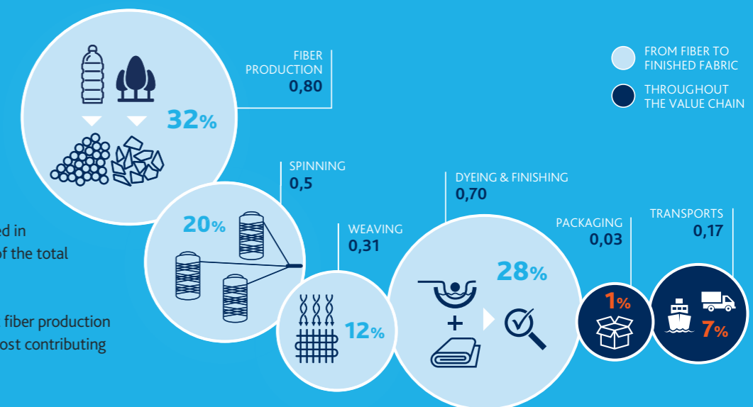
Figure 5. Climate impact per processing step for EG 260.
